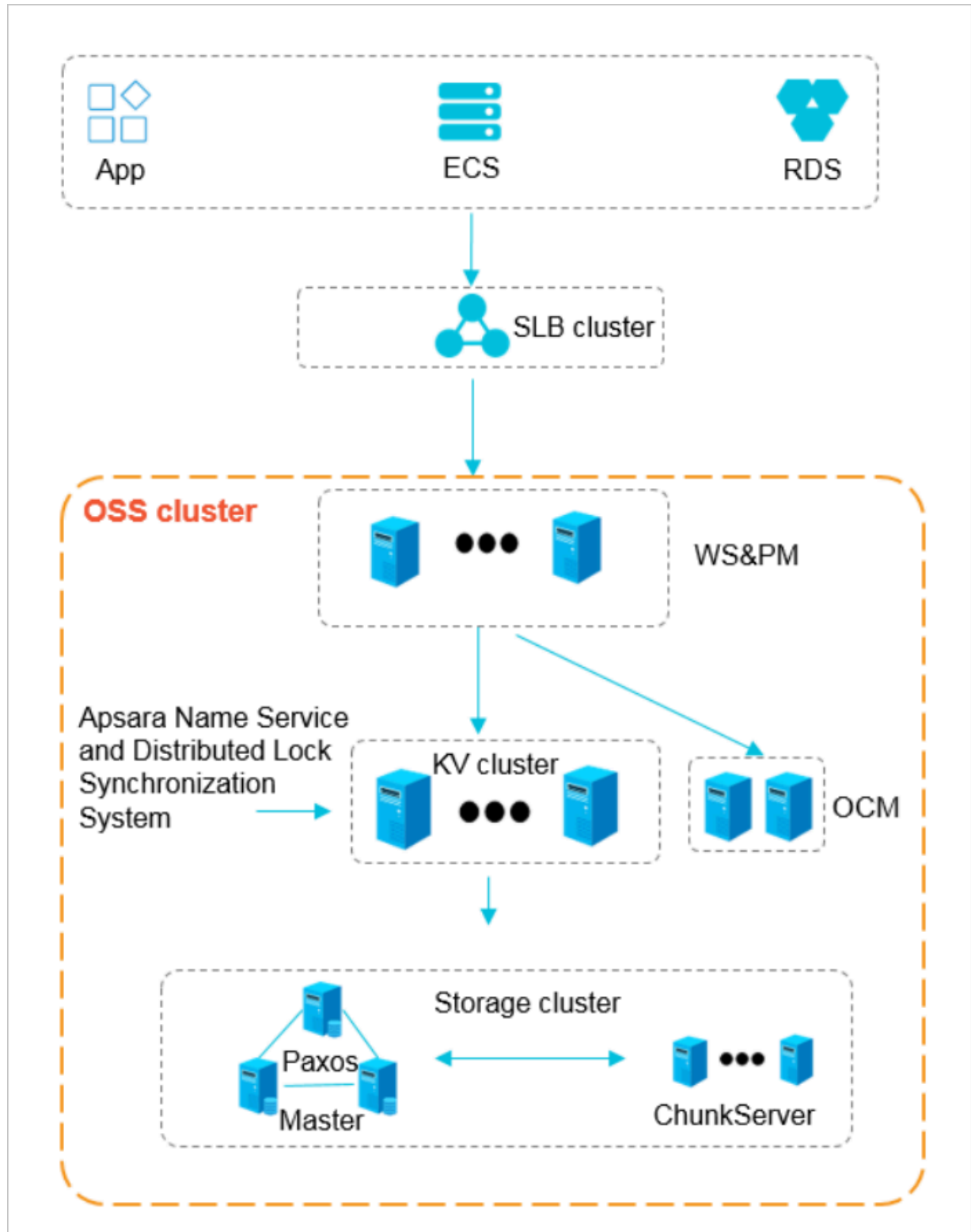
Figure 2-1: OSS architecture
