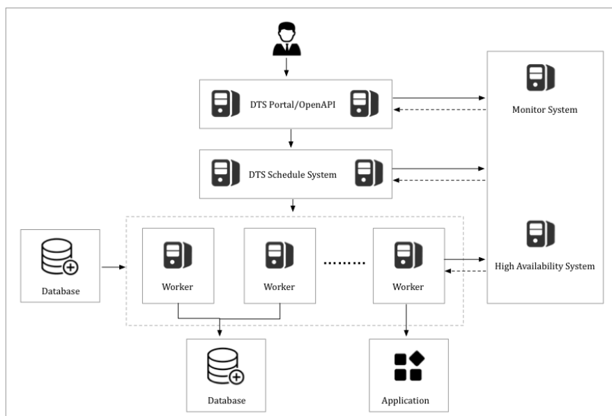
Figure 4-1: System architecture
