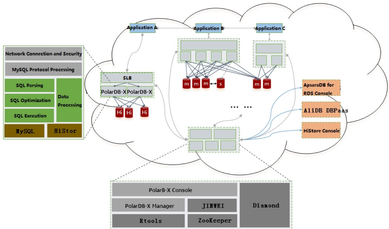
Figure 5-1: Figure of PolarDB-X architecture
