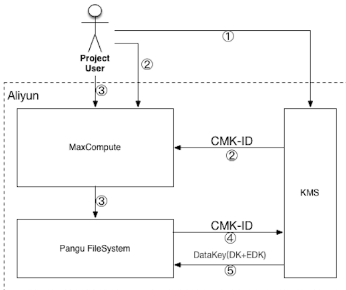
Figure 5-4: Data encryption process
