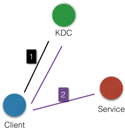
Figure 5-6: Principle of Kerberos authentication
