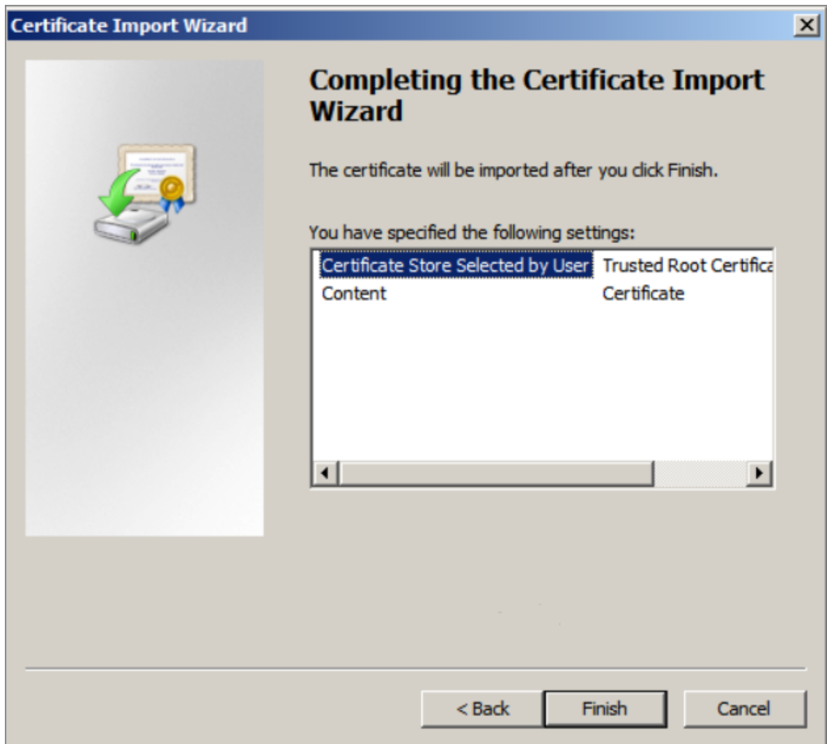
Figure 12-19: Import completed
