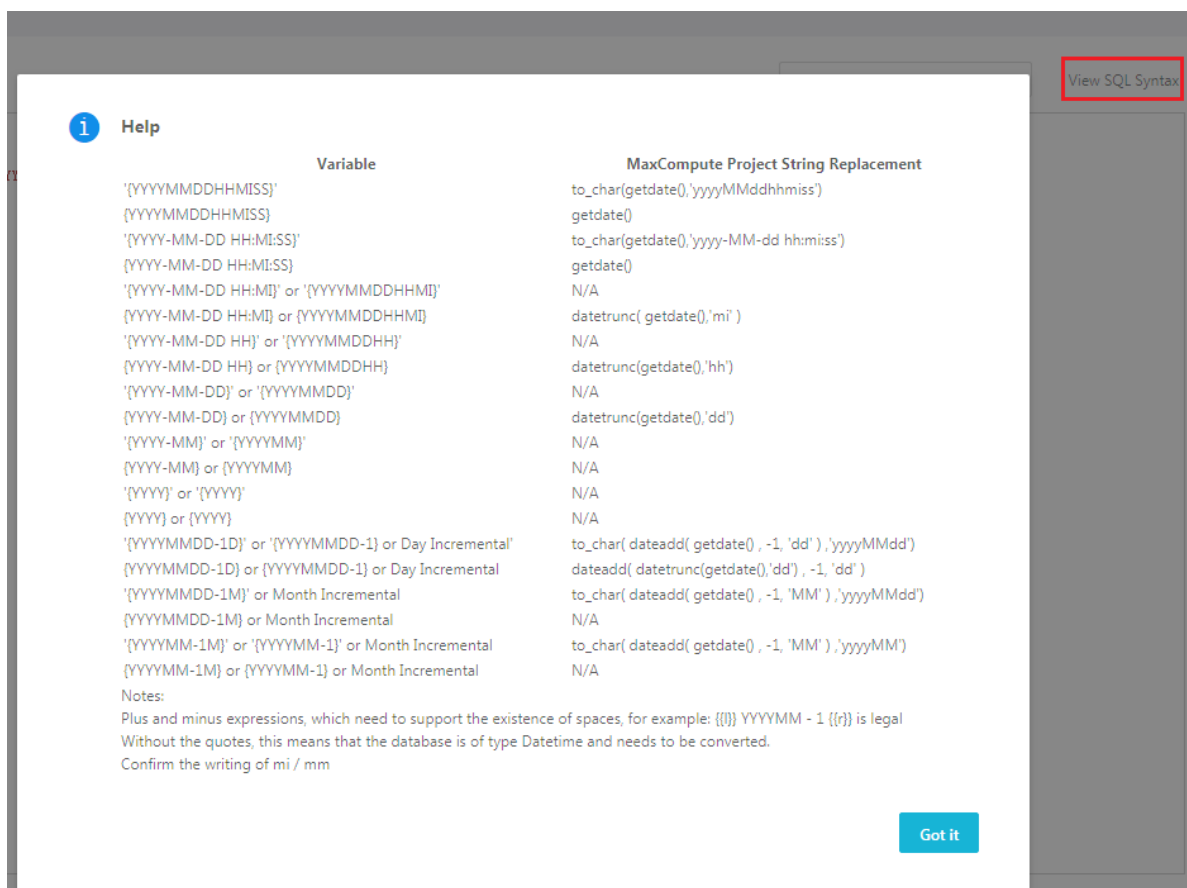
Figure 26-23: SQL rules
