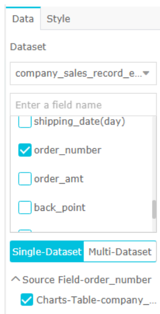
Figure 26-78: Filter conditions
