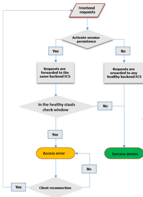
Figure 20-5: Request forwarding
