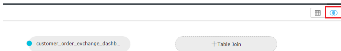
Figure 26-32: Data joining
