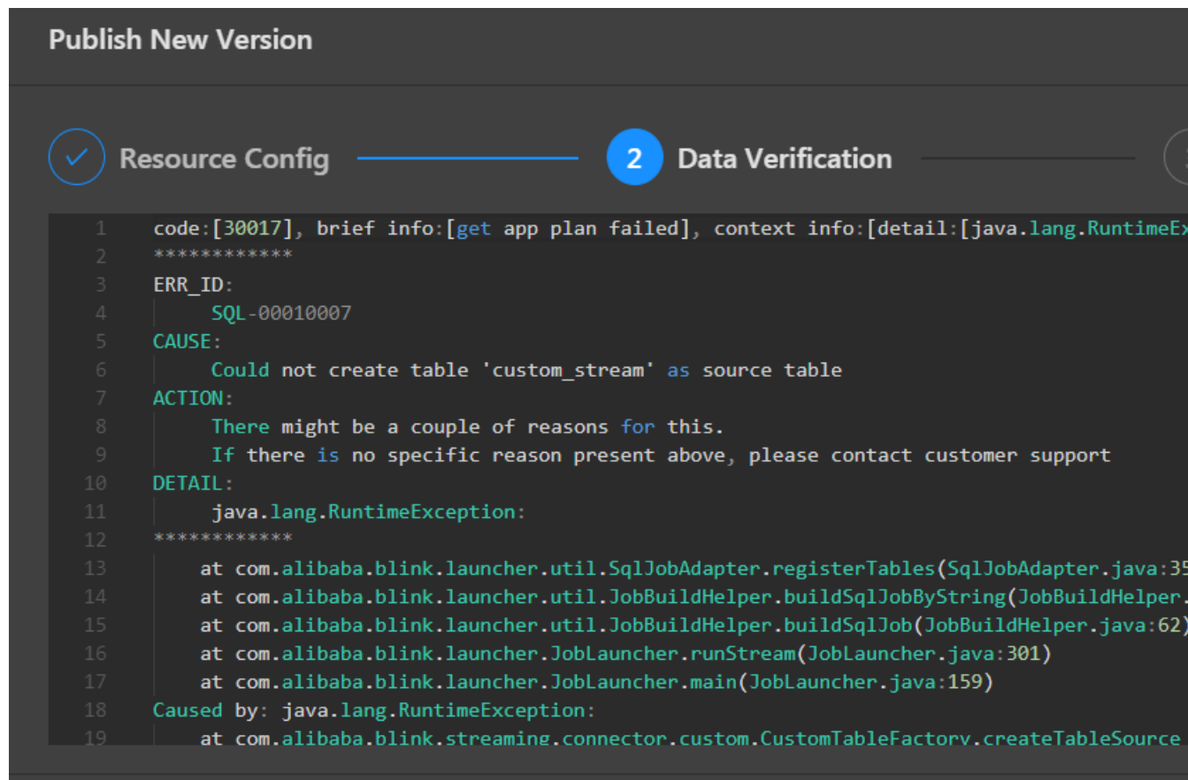
Figure 24-16: Data check
