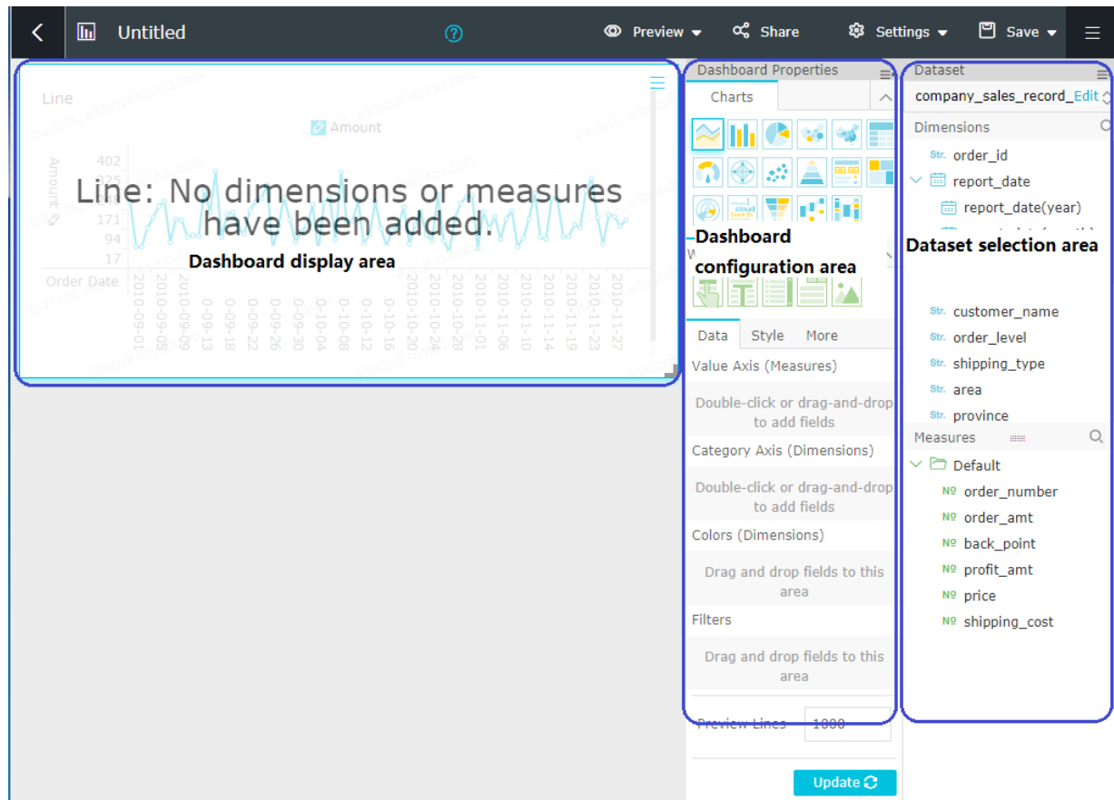
Figure 26-59: Dashboard
