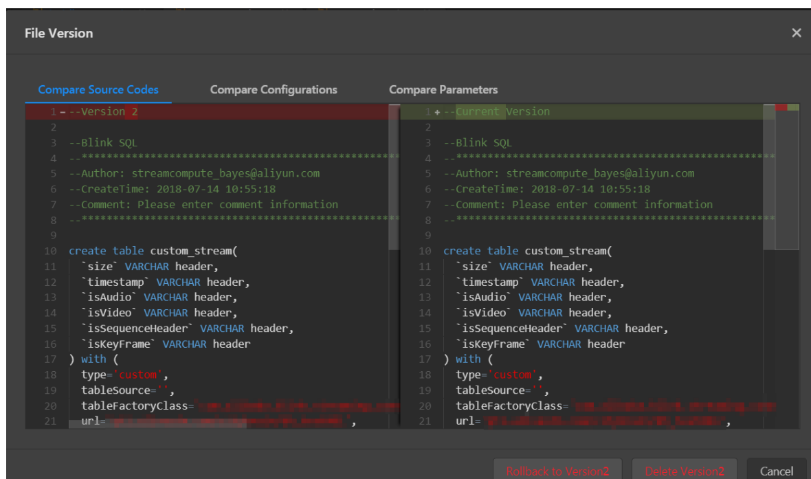
Figure 24-13: Code comparison
