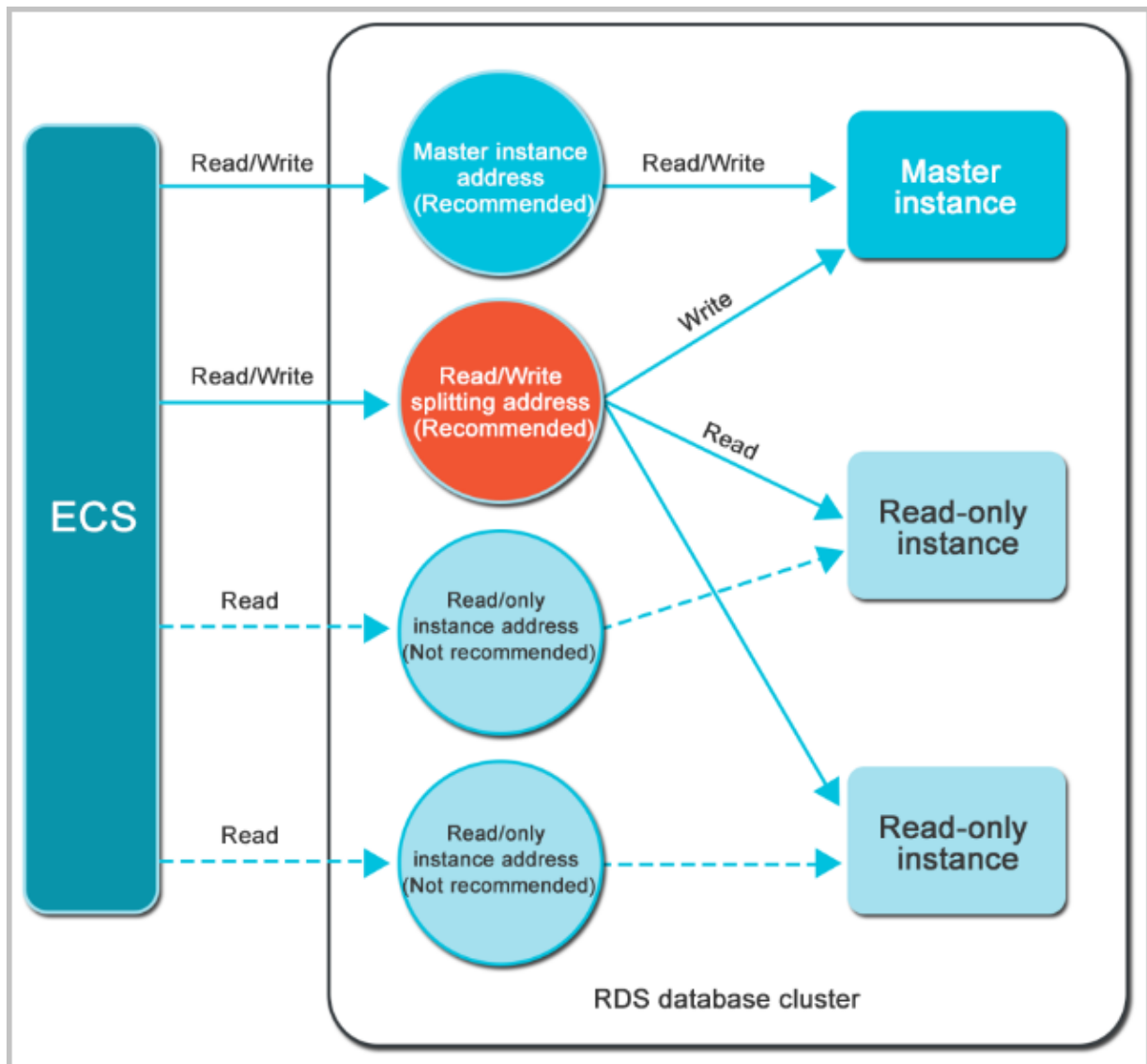
Figure 16-18: Principle of read/write splitting
