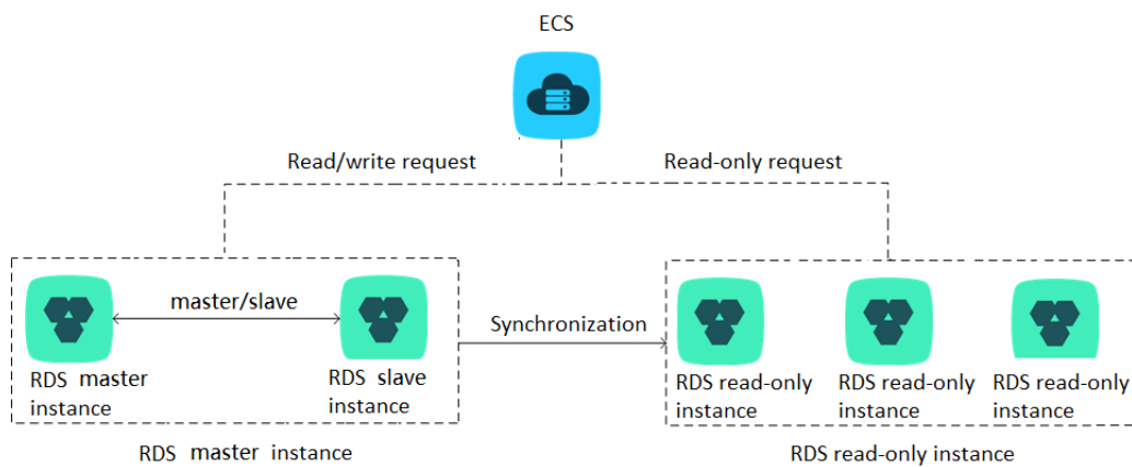
Figure 16-16: Topology of a read-only instance
