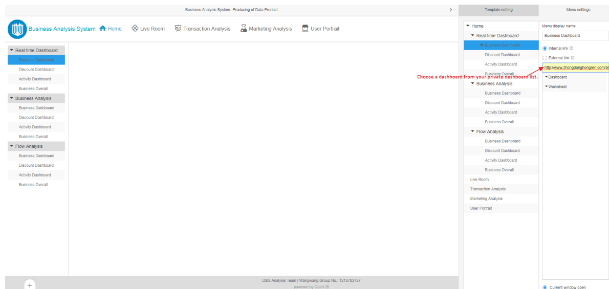
Figure 26-164: Menu settings
