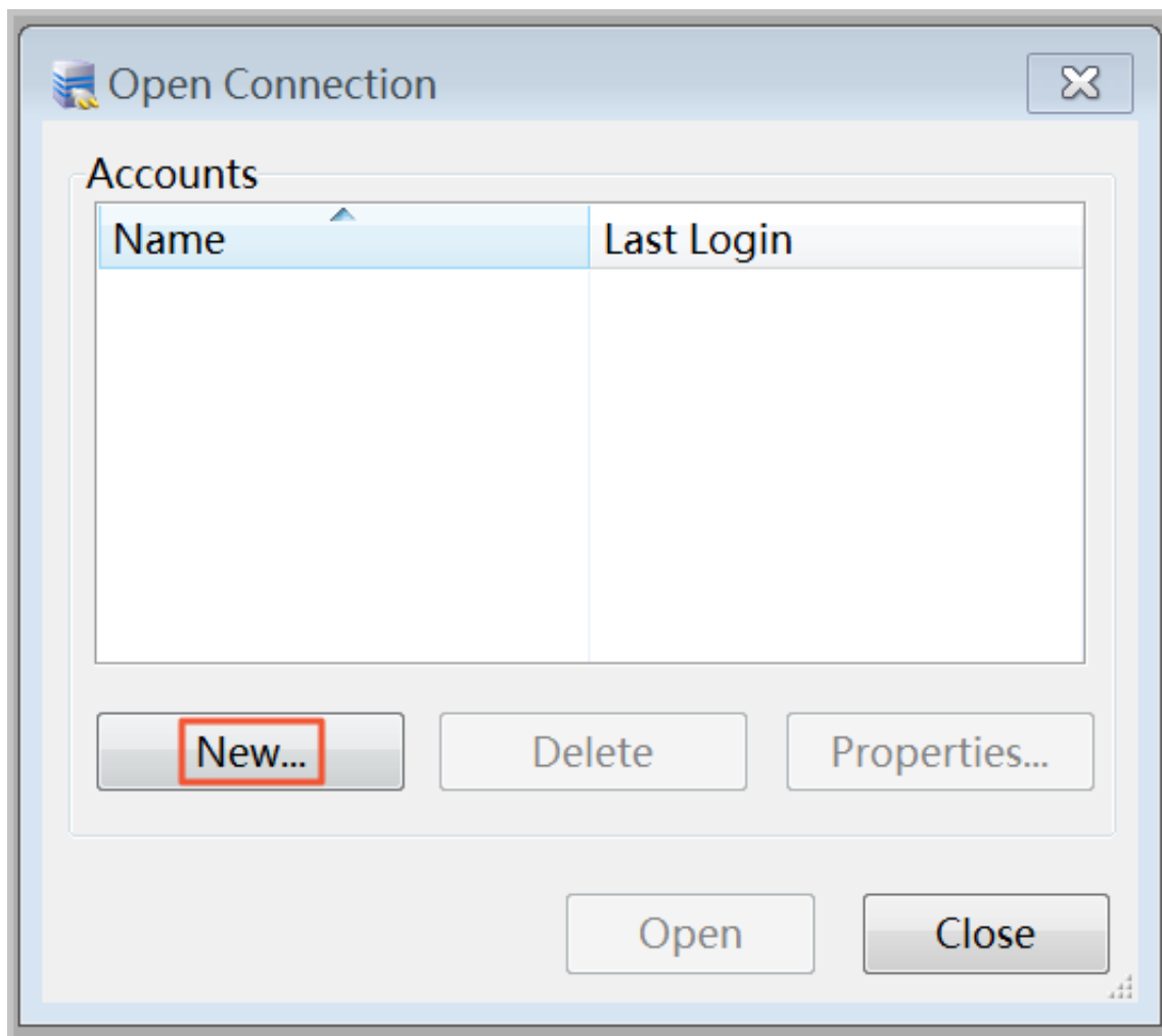
Figure 16-9: New connection
