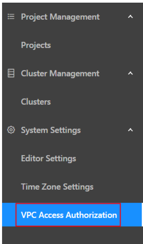
Figure 24-6: VPC authorization
