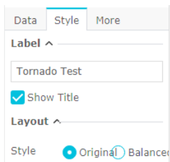
Figure 26-133: Chart layouts
