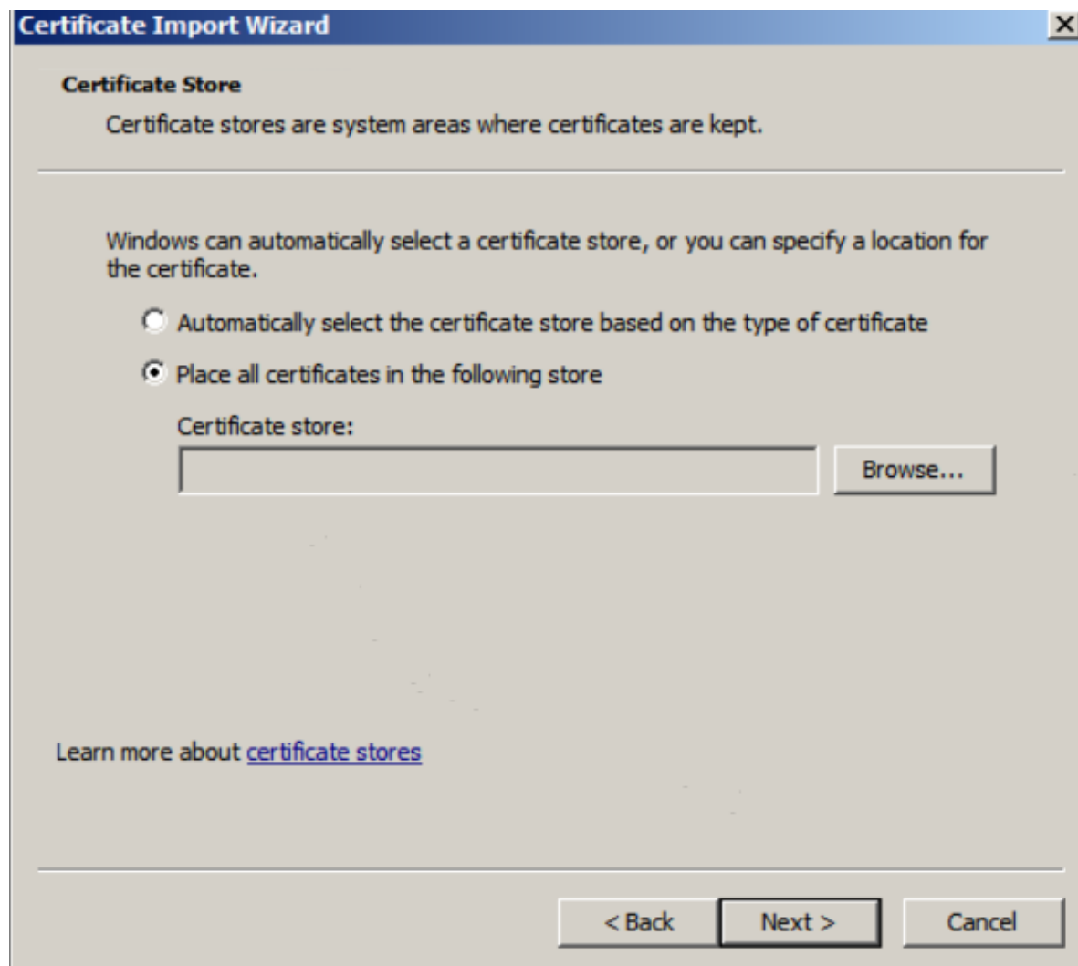
Figure 12-17: Store certificates
