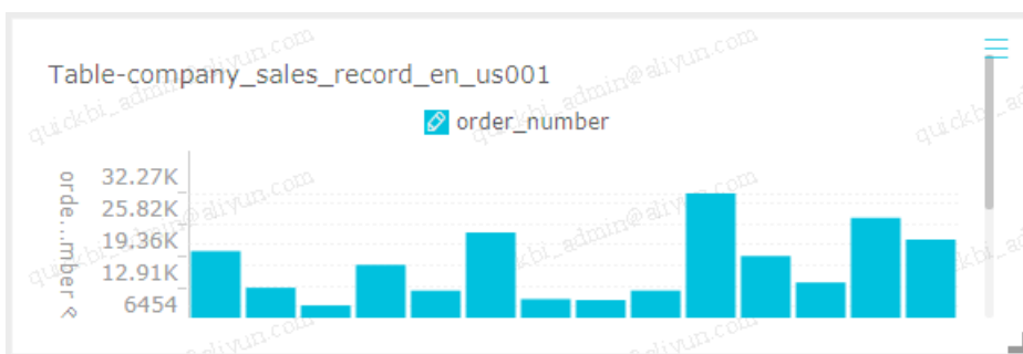
Figure 26-84: Query results
