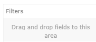
Figure 26-56: Filter
