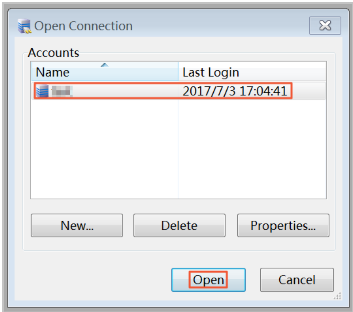
Figure 16-11: Instance connection
