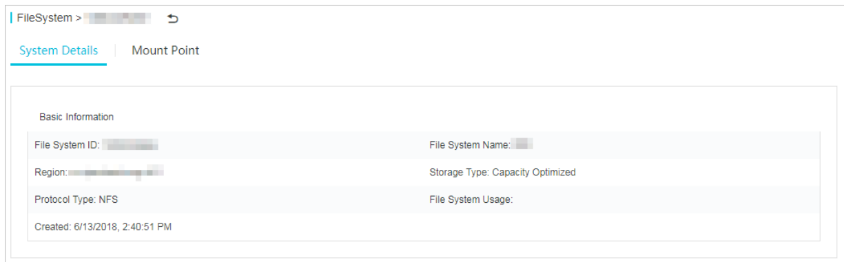
Figure 15-2: Instance details
