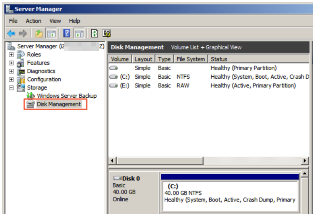
Figure 12-22: Manage disks
