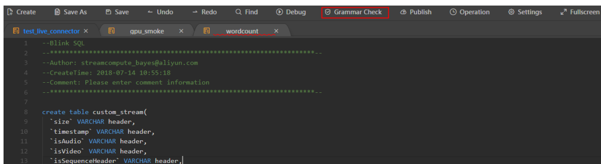
Figure 24-14: Syntax check
