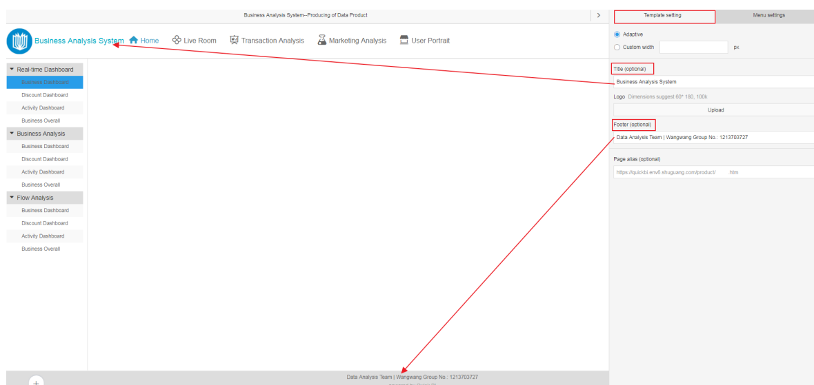
Figure 26-163: Template settings
