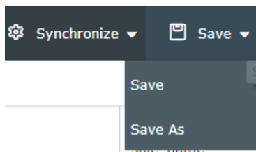
Figure 26-30: Save
