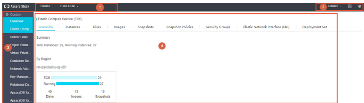
Figure 4-1: Web page
