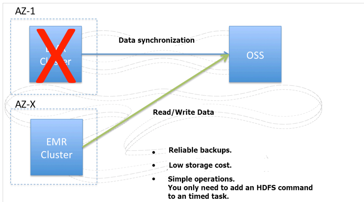
Figure 5-8: Data backup
