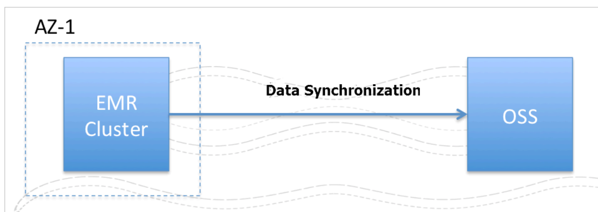
Figure 5-7: Data synchronization
