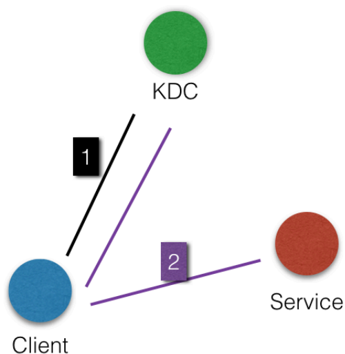
Figure 5-6: Kerberos authentication
